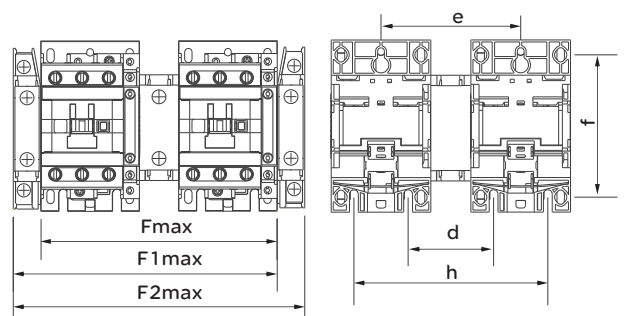
图8RDC5-40N~95N
