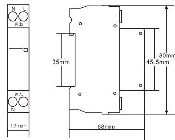
1P+N外形及安装尺寸
